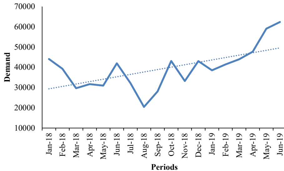
Figure 1. Scatter diagram of demand historical data
